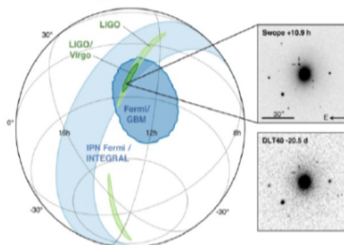
Figure 1. Localization of the gravitational-wave, gamma-ray, and optical signals. The left panel shows an orthographic projection of the 90% credible regions for LIGO (190 deg 2 ; light green), the initial LIGO-Virgo localization (131 deg 2 ; dark green), IPN triangulation from the time delay between Fermi and INTEGRAL (light blue), and Fermi-GBM (dark blue). The inset shows the location of the apparent host galaxy NGC 4993 in the Swope optical discovery image at 10.9 hr after the merger (top right) and the DLT40 pre-discovery image from 28.5 days prior to merger (bottom right). The reticle marks the position of the transient in both images.
